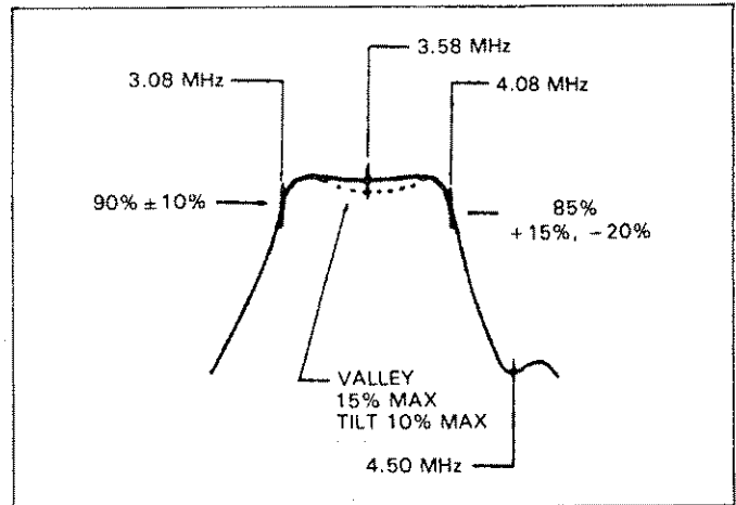
Fig. 21. Frequency Response Measurement.
