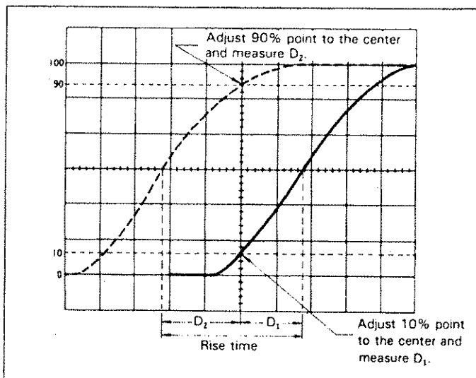
Fig. 13. Rise Time and Fall Time Measurement.
