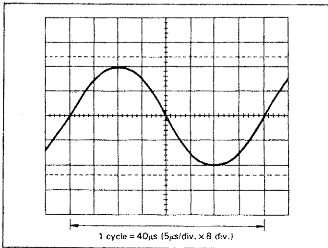
Fig. 9. Frequency Measurement.
