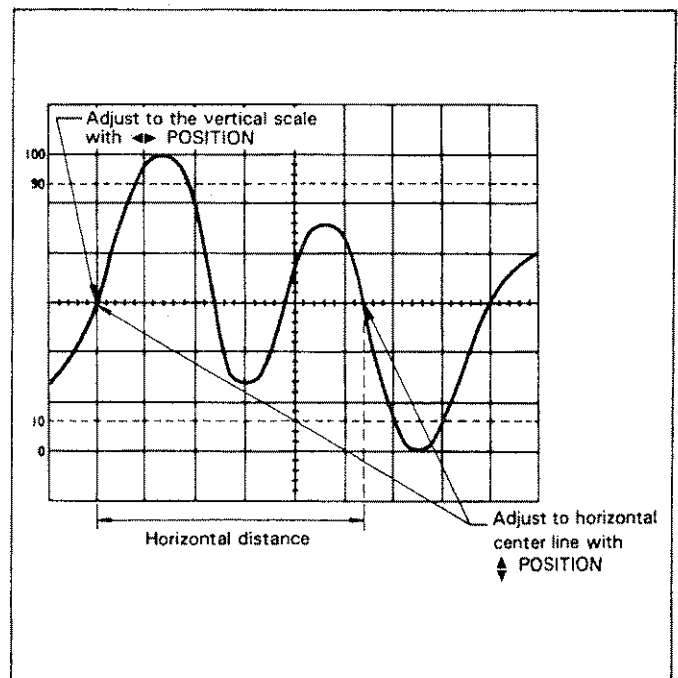
Fig. 8. Time Measurement.
